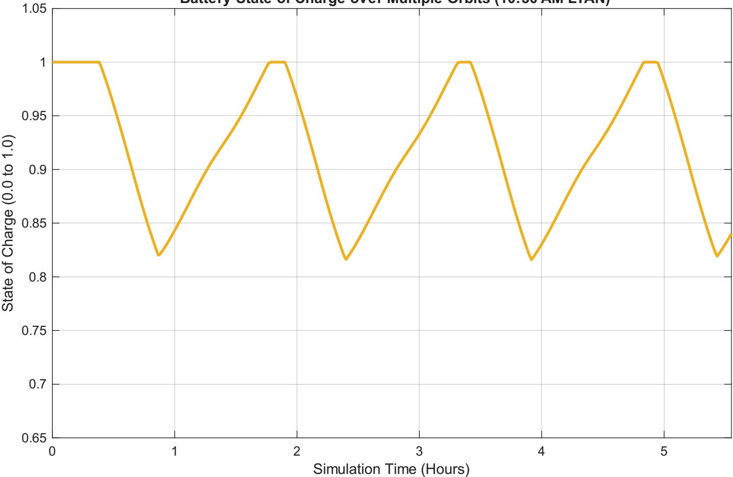
Battery State of Charge over Multiple Orbits (10:30 AM LTAN)
